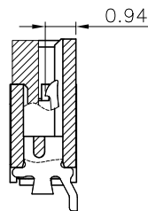
SECTION A-A Bottom Contact Side
