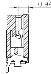
SECTION A-A Upper Contact Side.
